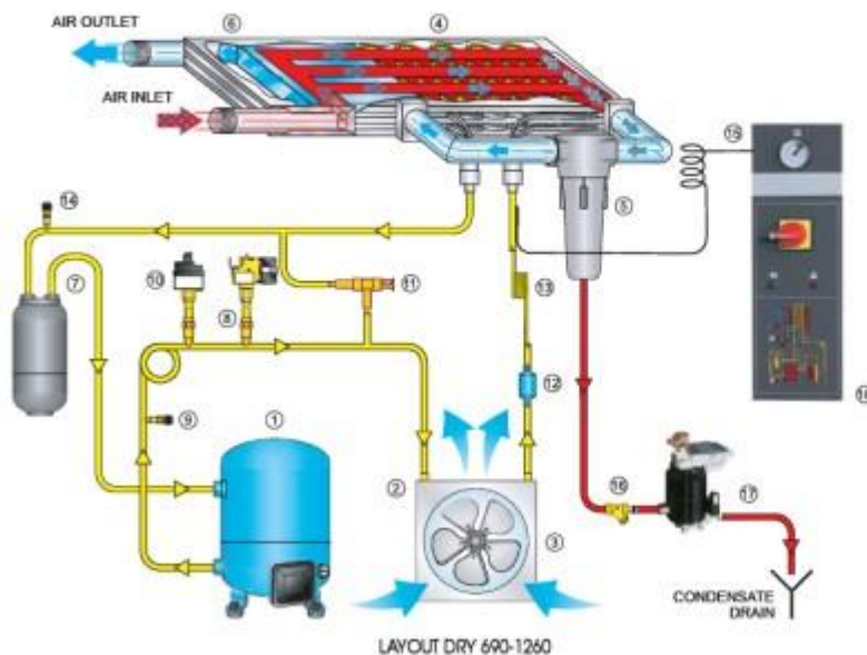
LAYOUT DRY 690-1250
